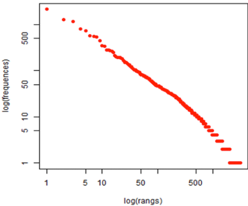
Figure 3: Statistics of the lexicographic analysis.
