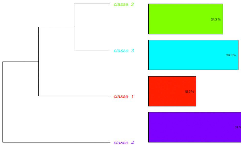
Figure 4: Dendrogram, including cluster analysis and lexical clusters.
