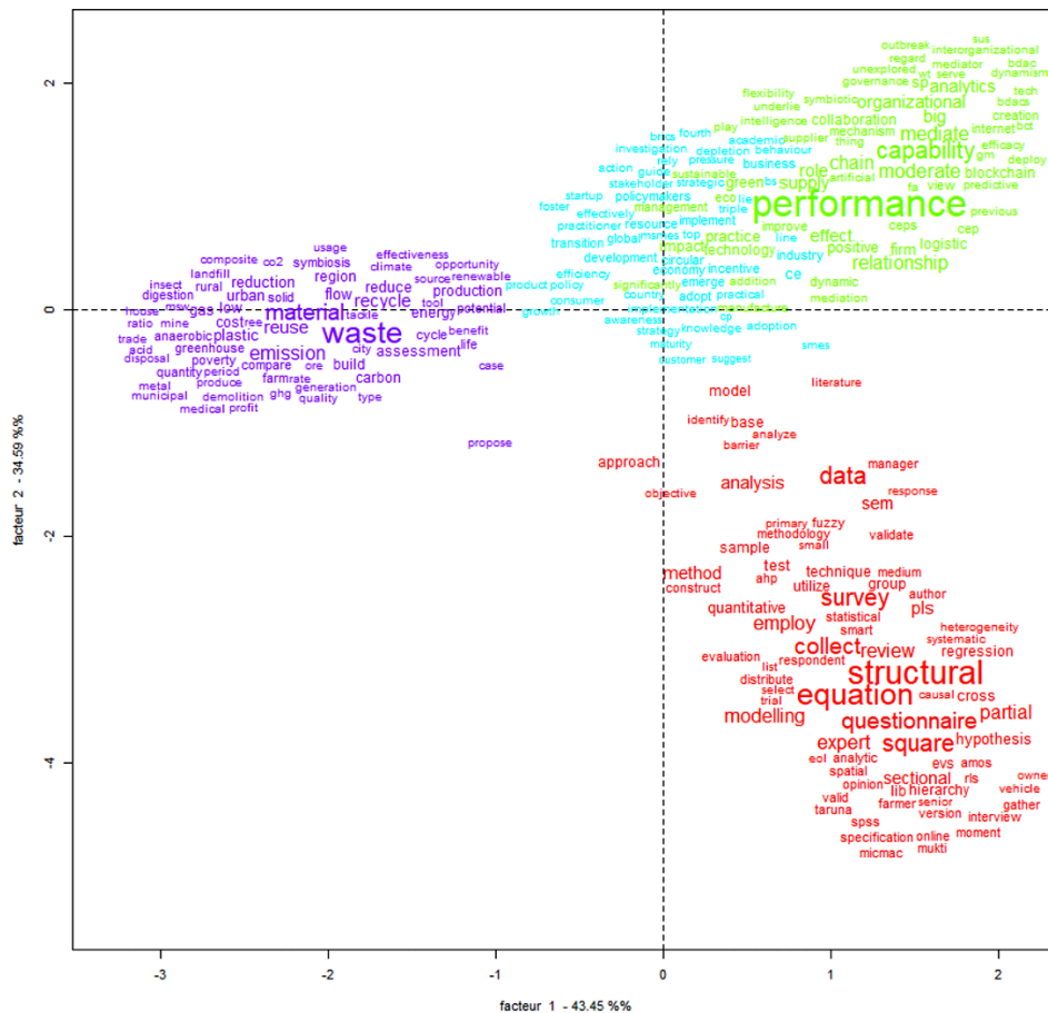
Figure 5: Factorial correspondence analyses (FCA) of frequently used words.
